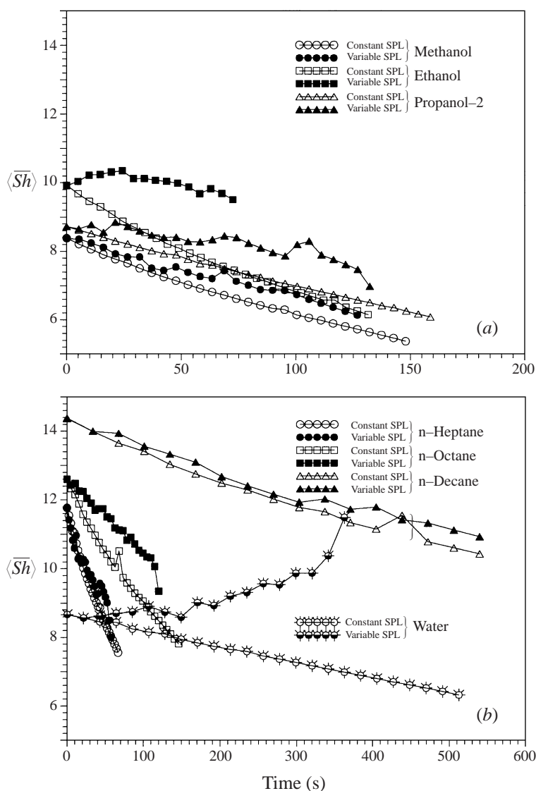
FIGURE 13. The Sherwood numbers for (a) methanol, ethanol and propanol-2 droplets and (b) n-heptane, n-octane, n-decane and water droplets with the initial volume of 3 \mu\text{l} as functions of time. Computations with constant and variable SPL. All values are larger than 2. Data obtained with variable SPL for water show an increase of \langle Sh \rangle with time.
